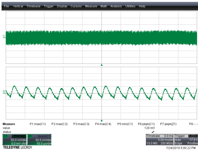
Figure 84 – Output Voltage Ripple. V_{IN} = 130 \text{ VDC} , I_{OUT} = 1.25 \text{ A} . Top Half: V_{OUT} , 50 mV / div. Bottom Half: Zoom @ 50 \mu\text{s} / div. V_{RIPPLE} = 120 \text{ mV}_{P-P}
