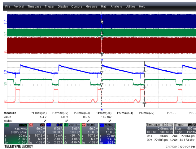
Figure 30 – Drain Voltage and Current Waveforms. V_{IN} = 550 \text{ VDC} , I_{OUT} = 2.5 \text{ A} . V_{DS(MAX)} = 131 \text{ V} , I_{DRAIN(MAX)} = 8.0 \text{ A} . Upper: I_{DRAIN} , 5 A, 2 ms / div. Middle: V_{GATE-SOURCE} , 5 V, 2 ms / div. Lower: V_{DRAIN-SOURCE} , 50 V, 2 ms / div. Bottom Half: Zoom @ 10 \mu\text{s} / div.
