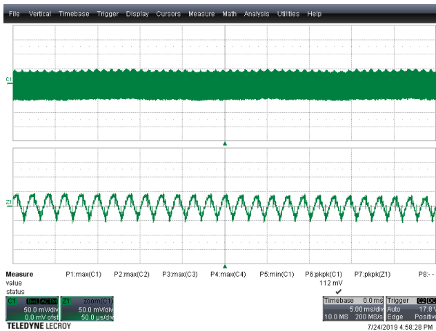
Figure 78 – Output Voltage Ripple. V_{IN} = 130 \text{ VDC} , I_{OUT} = 2.5 \text{ A} . Top Half: V_{OUT} , 50 mV, 5 ms / div. Bottom Half: Zoom @ 50 \mu\text{s} / div. V_{RIPPLE} = 112 \text{ mV}_{P-P}
