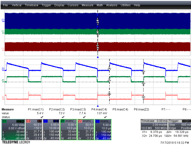
Figure 28 – Drain Voltage and Current Waveforms. V_{IN} = 130 \text{ VDC} , I_{OUT} = 2.5 \text{ A} . V_{DS(MAX)} = 73 \text{ V} , I_{DRAIN(MAX)} = 7.7 \text{ A} . Upper: I_{DRAIN} , 5 A, 2 ms / div. Middle: V_{GATE-SOURCE} , 5 V, 2 ms / div. Lower: V_{DRAIN-SOURCE} , 50 V, 2 ms / div. Bottom Half: Zoom @ 10 \mu\text{s} / div.
