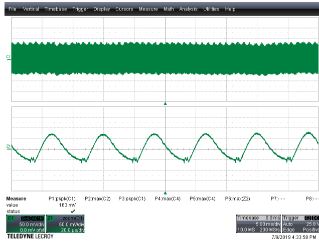
Figure 67 – Output Voltage Ripple. V_{IN} = 550 \text{ VDC} , I_{OUT} = 2.5 \text{ A} . Top Half: V_{OUT} , 50 mV, 5 ms / div. Bottom Half: Zoom @ 20 \mu\text{s} / div. V_{RIPPLE} = 163 \text{ mV}_{P-P}
