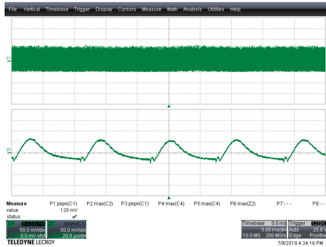
Figure 72 – Output Voltage Ripple. V_{IN} = 550 \text{ VDC} , I_{OUT} = 2.5 \text{ A} . Top Half: V_{OUT} , 50 mV, 5 ms / div. Bottom Half: Zoom @ 20 \mu\text{s} / div. V_{RIPPLE} = 128 \text{ mV}_{P-P}
