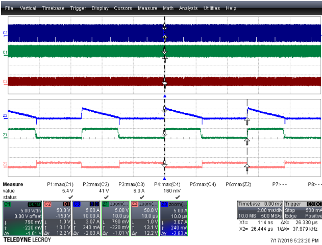
Figure 26 – Drain Voltage and Current Waveforms. V_{IN} = 30 \text{ VDC} , I_{OUT} = 0.85 \text{ A} . V_{DS(MAX)} = 41 \text{ V} , I_{DRAIN(MAX)} = 6.0 \text{ A} . Upper: I_{DRAIN} , 5 A, 2 ms / div. Middle: V_{GATE-SOURCE} , 5 V, 2 ms / div. Lower: V_{DRAIN-SOURCE} , 50 V, 2 ms / div. Bottom Half: Zoom @ 10 \mu\text{s} / div.
